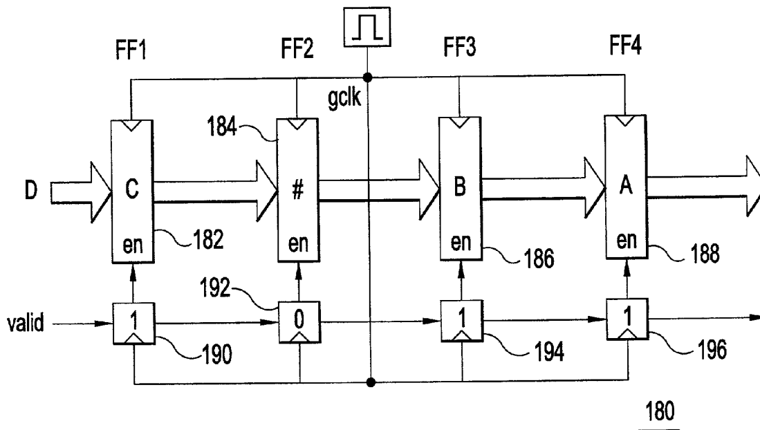
FIG.5 (PRIOR ART)
